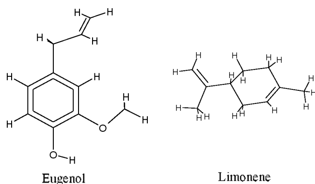
Figure 1. Structures of two typical essential oils.
