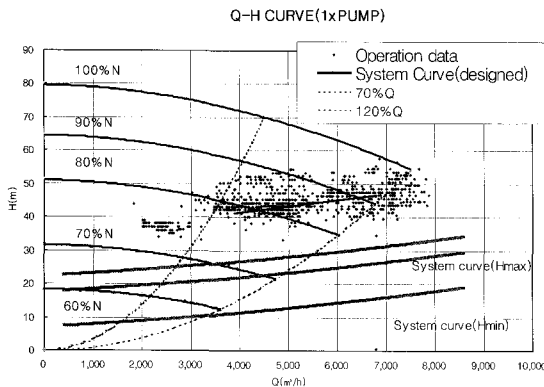
Fig. 10 Q-H curves (1 x pump)
