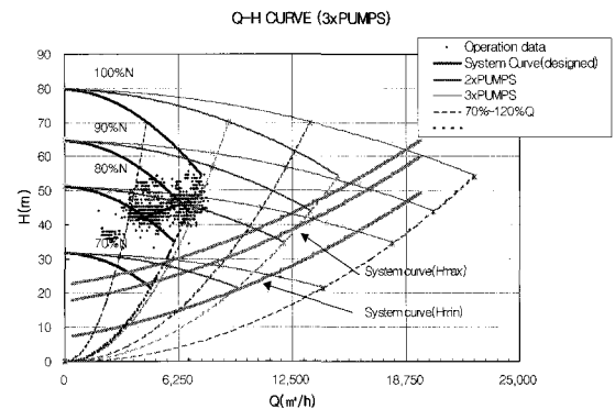
Fig. 11 Q-H curves (3 x pumps)
