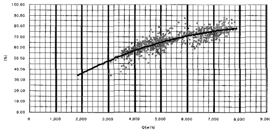
Fig. 5 Flow rates vs pump efficiency
