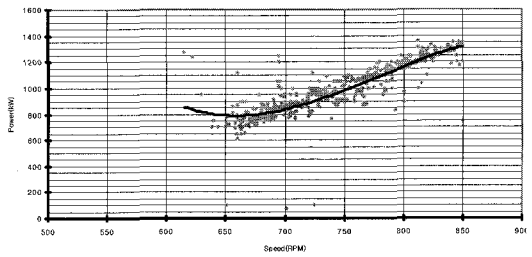
Fig. 8 Rotating speed vs power
