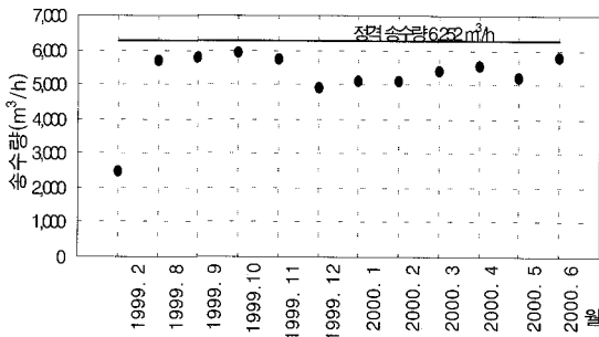
Fig. 1 Variation of monthly supply flow rate
