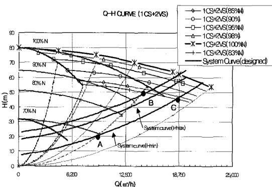
Fig. 12 Q-H curves (1CS + 2VS)
