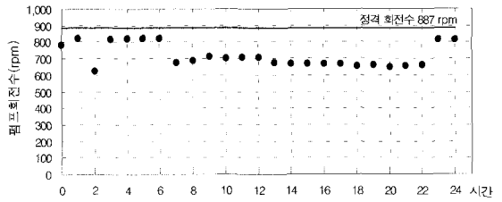
Fig. 4 Variation of timely rotating speed
