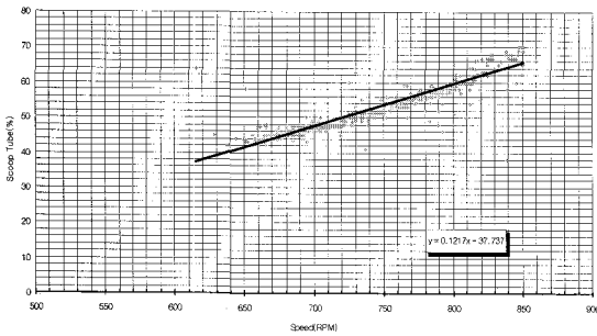
Fig. 9 Rotating speed vs scoop tube opening
