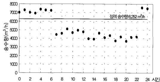
Fig. 2 Variation of timely supply flow rate
