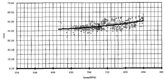
Fig. 7 Rotating speed vs total head
