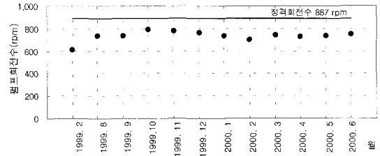
Fig. 3 Variation of monthly rotating speed
