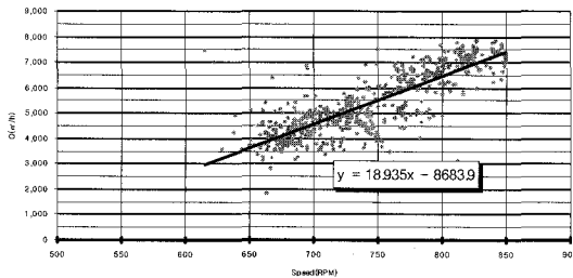
Fig. 6 Rotating speed vs flow rate
