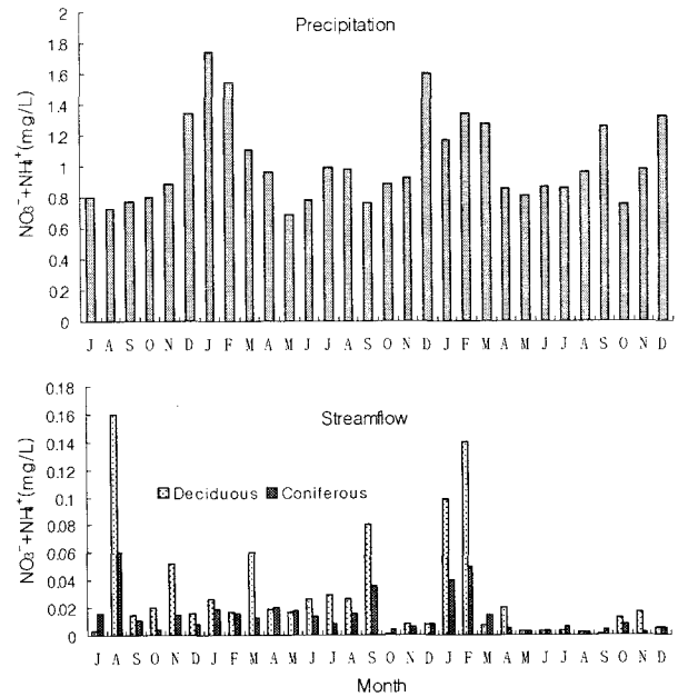
Fig. 2. Monthly concentration(mg/L) of \text{N}(\text{NO}_3^- + \text{NH}_4^+) in precipitation and streamflow in deciduous and coniferous forest watershed ecosystems from July 1991 to December 1993.
