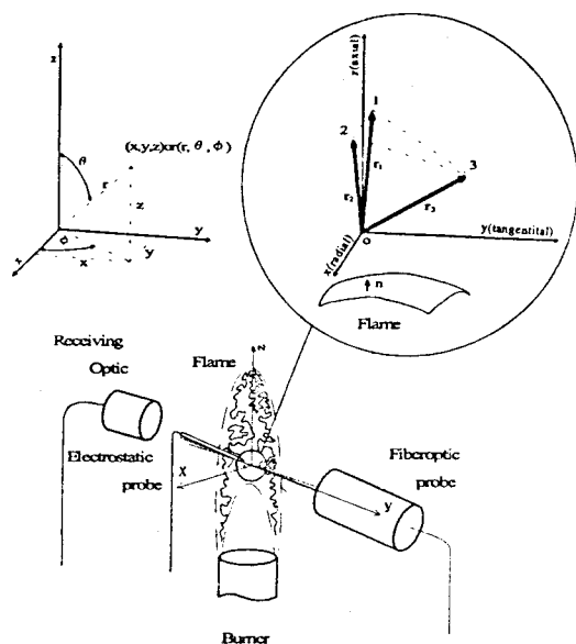
Fig. 1 Simultaneous measurement of the local gas velocity and the local flame front movement
