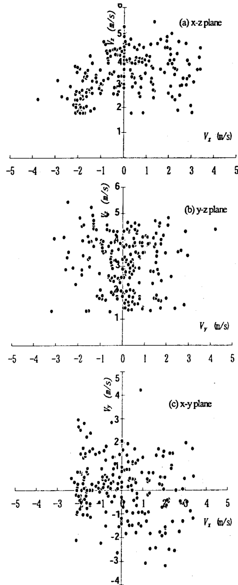
Fig. 2 A vector distribution map of the local flame-front velocity in (a) the x-z plane, (b) the y-z plane and (c) the x-y plane
