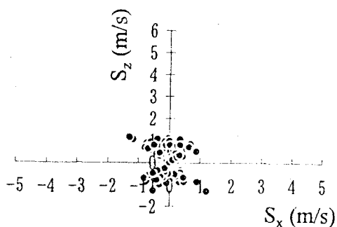
Fig. 4 A vector distribution map of the component in the x-z plane of the local velocity of the flamelet with respect to the gas
