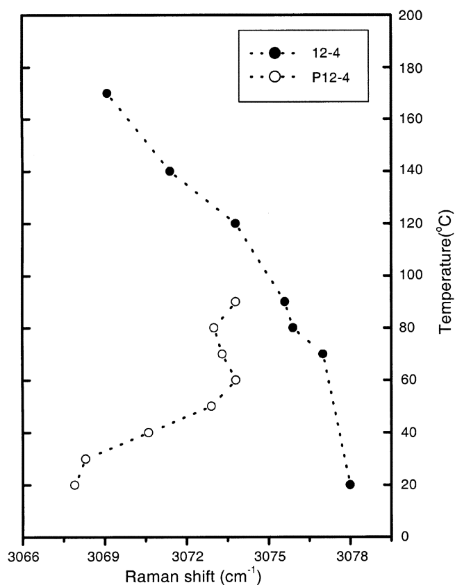
Figure 2. Temperature dependence of the C-H stretching modes for P12-4 (○) and 12-4 (●).
