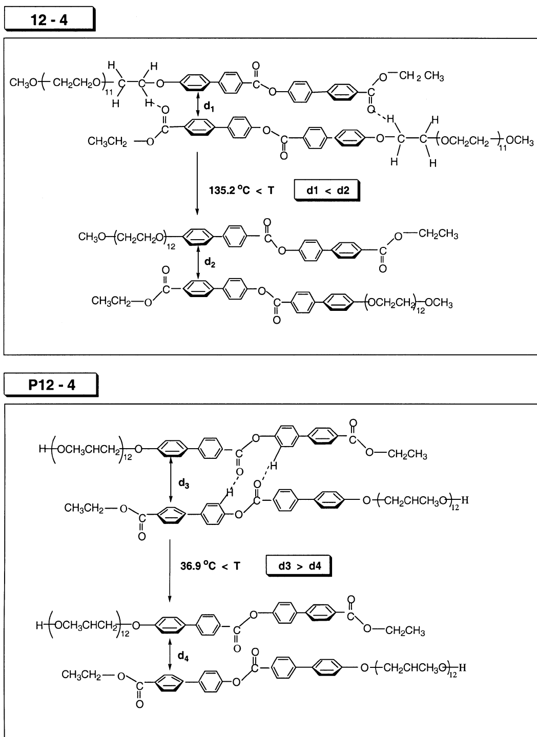
Figure 4. Schematic diagram for the intermolecular arrangements of P12-4 and 12-4 before and after the phase transition temperatures. The distance between neighboring mesogens is designated by d_i ( i = 1, 2, 3, 4 ).
