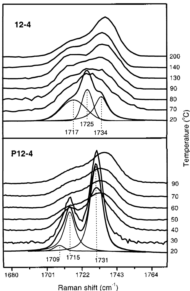
Figure 1. Temperature dependence of the carbonyl modes for P12-4 (bottom) and 12-4 (top). The three solid lines are obtained through curve-fitting of the corresponding spectrum at 20 °C.
