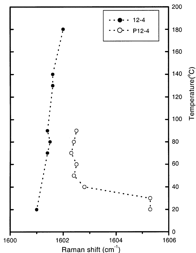
Figure 3. Temperature dependence of the C=C stretching modes for P12-4 (○) and 12-4 (●).
