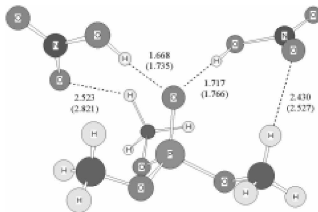
Figure 2. Structure of TMP-(HNO 3 ) 2 optimized at the MP2 and HF levels using 6-31G(d,p) basis sets. Bond lengths are in Å. Numbers in parenthesis are obtained from the HF level.
