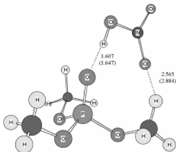
Figure 1. Structure of TMP-HNO 3 optimized at the MP2 and HF level using 6-31G(d,p) basis sets. Bond lengths are in Å. Numbers in parenthesis are obtained from the HF level.
