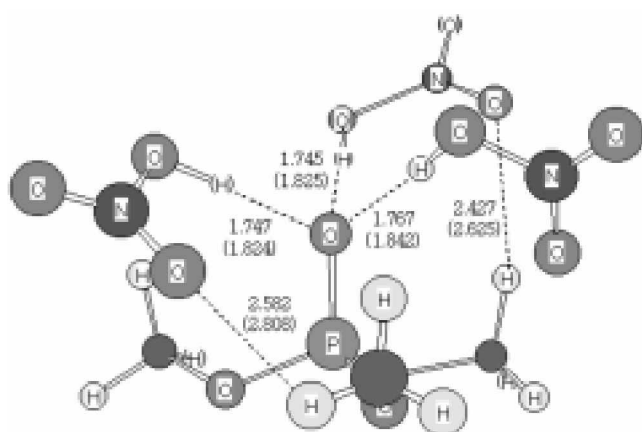
Figure 3. Structure of TMP-(HNO 3 ) 3 optimized at the MP2 and HF levels using 6-31G(d,p) basis sets. Bond lengths are in Å. Numbers in parenthesis are obtained from the HF level.
