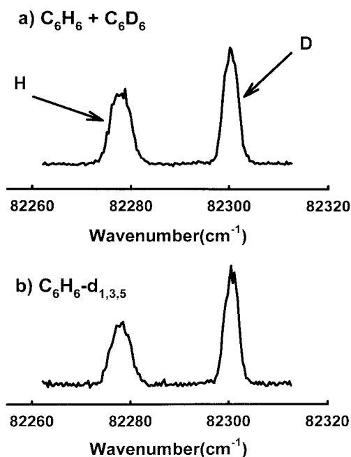
Figure 1. H(D) atom spectra from photodissociation of (a) 1:1 mixture of benzene and benzene- d_6 (b) 1,3,5-benzene- d_3 at 243 nm.
