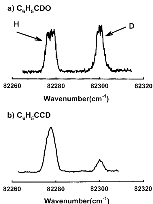
Figure 2. H(D) atom spectra from photodissociation of (a) C_6H_5CDO and (b) C_6H_5CCD at 243 nm.
