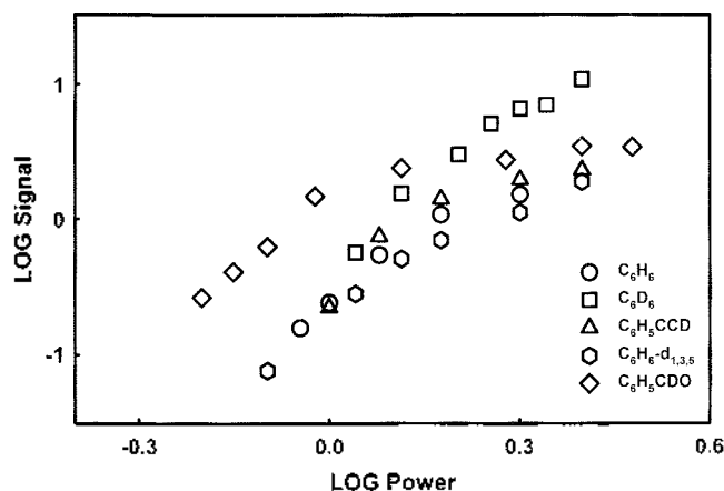
Figure 3. log-log plots of H(D) atom signals vs. laser intensities produced from the photodissociation of benzene, phenylacetylene, and benzaldehyde at 243 nm. The plots show linear slopes of 4.2 \pm 0.3 at the low laser intensities.
