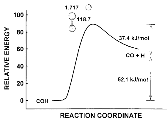
Figure 4. Potential energy curve along the minimum energy path obtained by ab initio calculations for the H atom elimination reaction from COH. The transition state geometry is depicted on top of the potential energy maximum.
