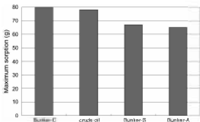
Figure 8. Maximum sorption capacity of the exfoliated graphite for different grade heavy oil.
