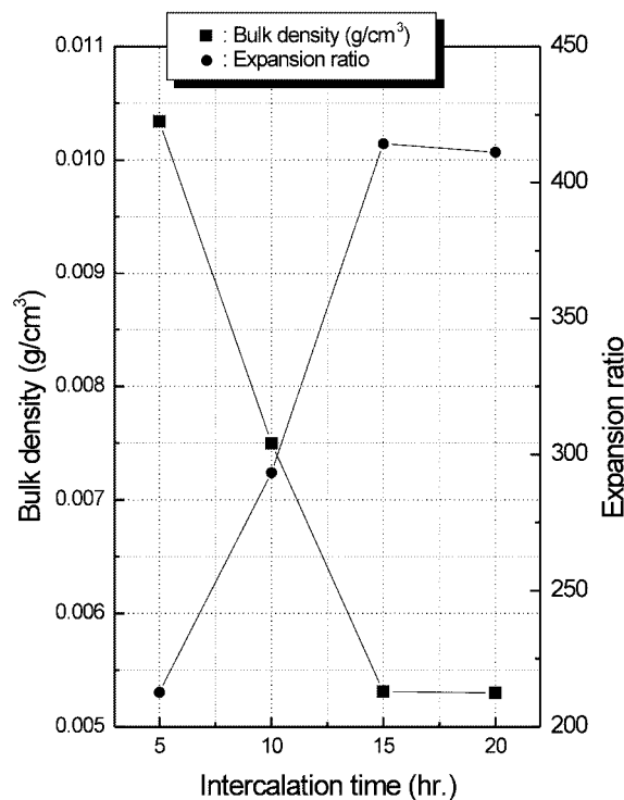
Figure 5. Bulk density and expansion ratio of the exfoliated graphite depending on the reaction temperature.
