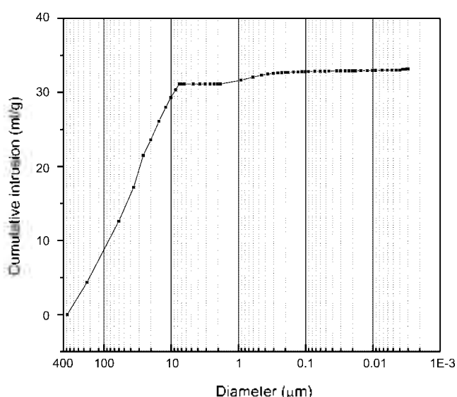
Figure 6. Pore characteristic of the exfoliated graphite by the mercury porosimetry.
