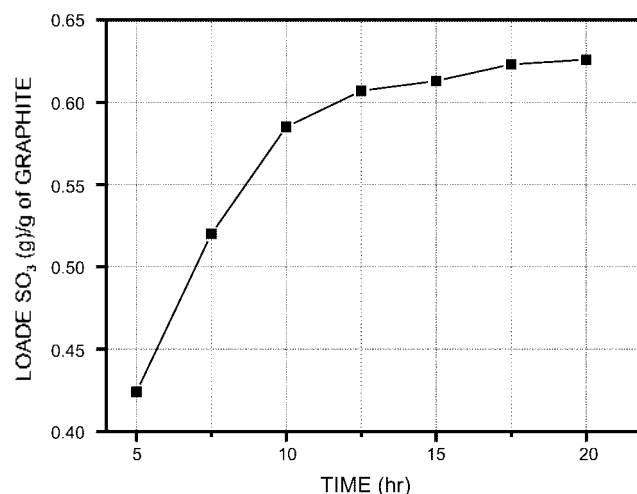
Figure 2. Loaded \text{SO}_3 gas per g-graphite depending on the reaction time.
