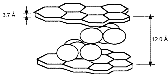
Figure 4. Schematic draws for the hypothetical configuration of \text{SO}_3 molecules in the graphite interlayer.
