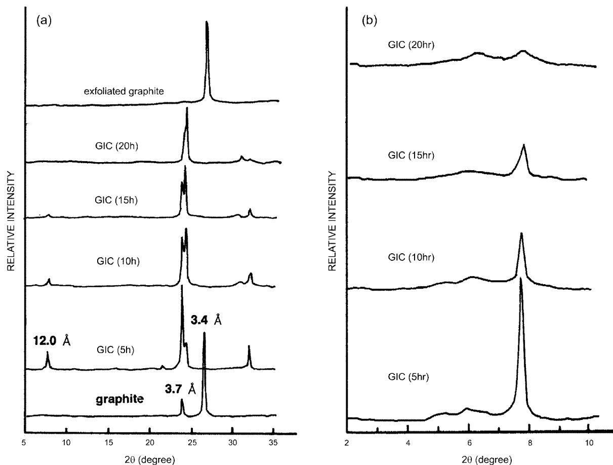
Figure 3. X-ray diffraction patterns of the \text{SO}_3 intercalated graphite at various reaction times: (a) 2\theta : 5-35, (b) \theta : 2-10.
