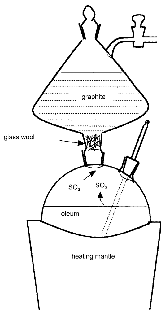
Figure 1. Reaction equipment for the reaction between graphite and \text{SO}_3 gas.
