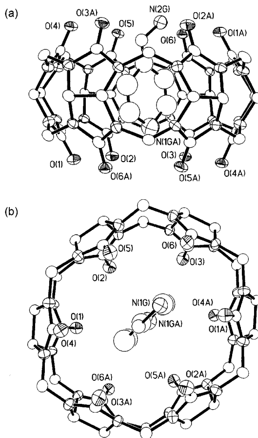
Figure 2. X-ray crystal structure of 7 : (a) side view and (b) top view. Hydrogen atoms, counter anions ( \text{Br}^- ), and solvent ( \text{H}_2\text{O} ) molecules are omitted for clarity. Hydrogen bonding interactions: \text{N2G}\cdots\text{O1A} 2.79(1)Å, \text{N2G}\cdots\text{O5} 3.05(1)Å, \text{N2G}\cdots\text{O6} 2.88(1)Å.
