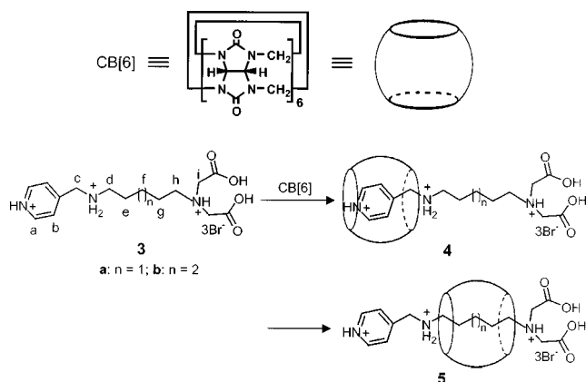
Scheme 2. Threading of CB[6] with the string 3 to form the kinetic product 4 and its conversion to the thermodynamic product 5 .
