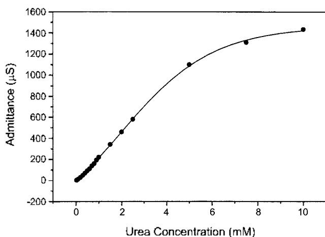
Figure 1. Calibration curve of the biosensor for urea in 5.0 mM imidazole-HCl buffer at pH 7.5.
