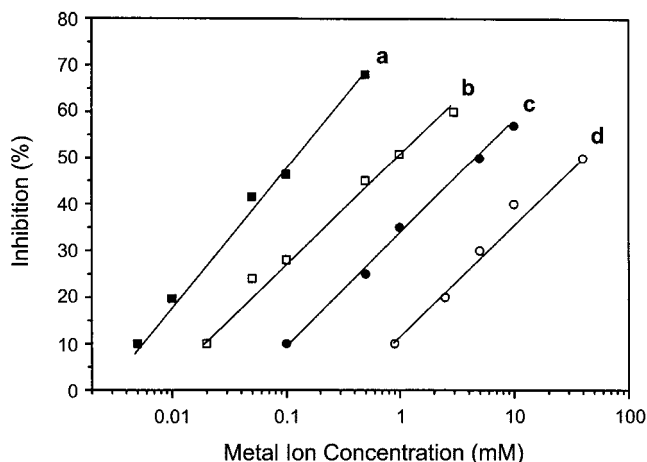
Figure 3. Calibration curve of the biosensor for the heavy-metal ion determination. The biosensor was pre-incubated in a test solution of metal ions for 10 min. The urea used was 1.0 mM. a, \text{Hg}^{2+} ; b, \text{Cu}^{2+} ; c, \text{Cd}^{2+} ; d, \text{Pb}^{2+}
