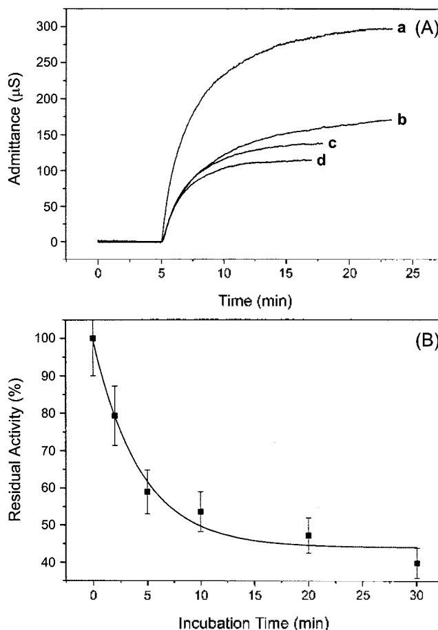
Figure 2. (A) The admittance responses for addition of 1.0 mM urea to the biosensor preincubated with 0.1 mM \text{Hg}^{2+} solution: a, no incubation; b, 5 min incubation; c, 10 min incubation; d, 20 min incubation (B) Residual biosensor activity vs incubation time. The response of the biosensor non-treated with metal ions was taken for 100%. Detailed conditions can be found in the experimental section.
