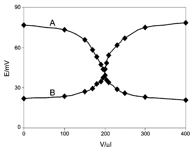
Figure 5. Potentiometric titration curves of 20.0 mL 1.0 \times 10^{-1} M solution of \text{Cu}^{2+} with 1.0 \times 10^{-2} M of EDTA (A), and 20.0 mL 1.0 \times 10^{-4} M solution of EDTA with 1.0 \times 10^{-2} M of \text{Cu}^{2+} (B).
