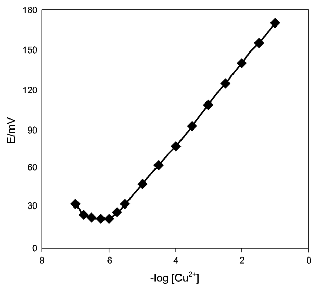
Figure 3. Calibration graph of copper(II) ion-selective electrode based on DIABE.
