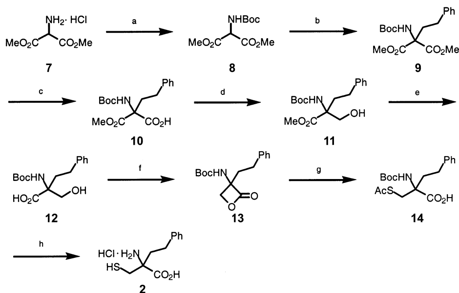
Scheme 2. (a) \text{Boc}_2\text{O} , \text{Et}_3\text{N} , \text{CH}_2\text{Cl}_2 ; (b) \text{NaH} , (2-iodoethyl)benzene, DMF, 100 °C, 2 h, 80%; (c) 1 N \text{NaOH} , \text{H}_2\text{O}/\text{THF} (5/1), rt, 4 h, 92%; (d) i) isobutyl chloroformate, \text{Et}_3\text{N} , THF, 0 °C, ii) \text{NaBH}_4 , 0 °C, 1 h, 71% (two steps); (e) \text{LiOH} , MeOH, rt, 1 day, 93%; (f) \text{Ph}_3\text{P} , DMAID, THF, -78 °C, 55%; (g) \text{AcSK} , DMF, rt, 30 min, 90%; (h) 6 N \text{HCl} , reflux, 2 h, 98%.
