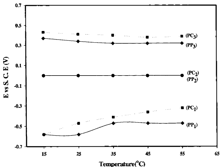
Fig. 3. Variation of potential as a function of temperature (°C): PPI-3: poly(propylene) waves; PCI-3: poly(carbonate) waves.
