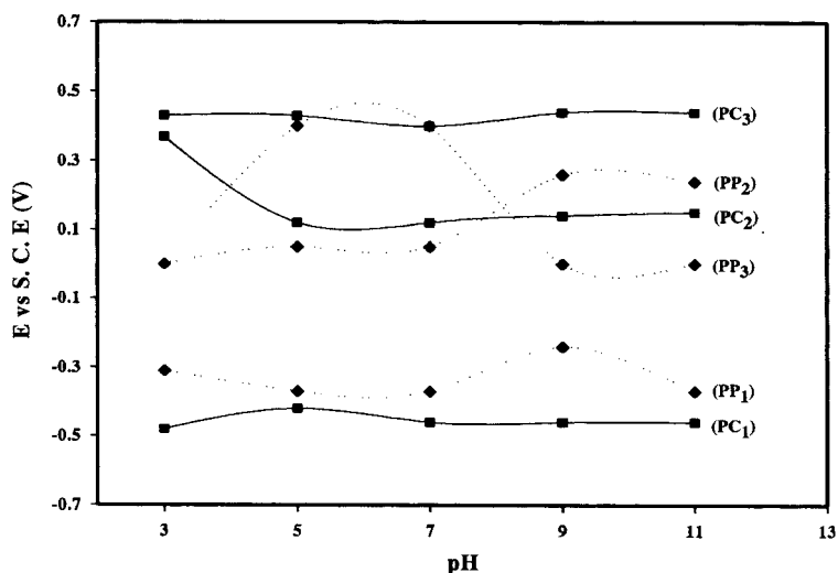
Fig. 5. Dependences of potential on pH: PP1-3: poly(propylene) waves; PC1-3: poly(carbonate) waves.
