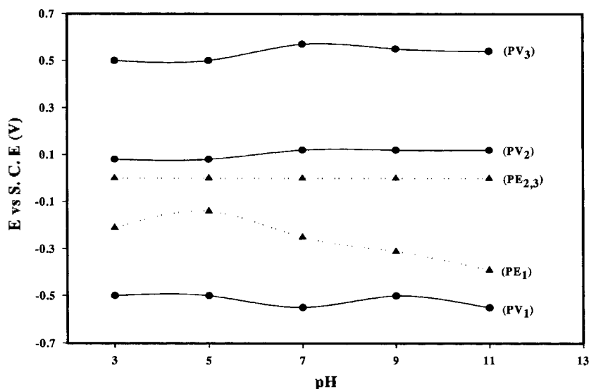
Fig. 4. Dependences of potential on pH: PV1-3: PVC waves; PE1-3: PET waves.
