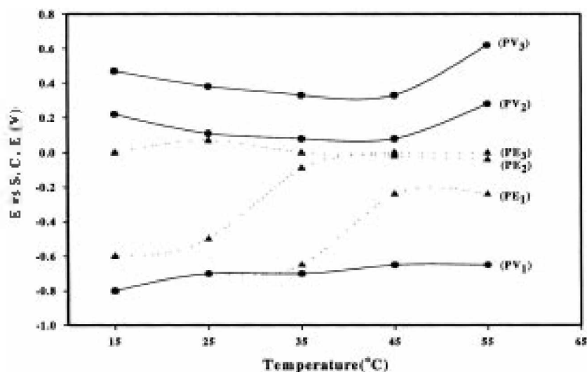
Fig. 2. Variation of potential as a function of temperature (°C).
