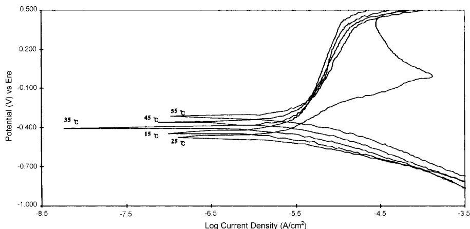
Fig. 1. Polarization curves of poly(carbonate) at various temperatures.
