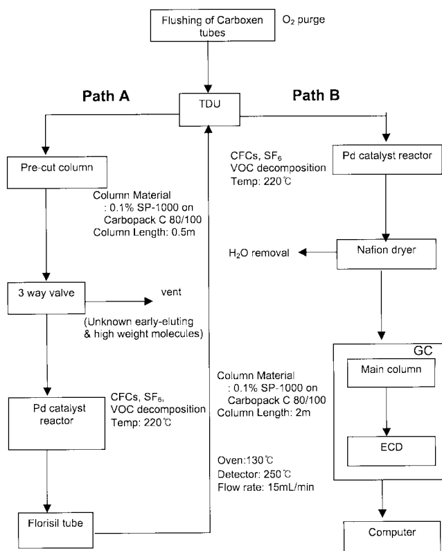
Figure 2. Schematic diagram of PFC analysis system: Path A: refocusing process, Path B: analysis process.
