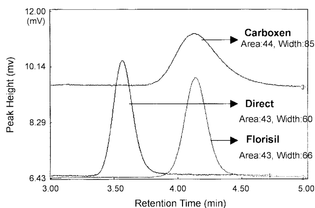
Figure 4. Variation of PMCH peak widths depending on sampling tube inner diameter.
