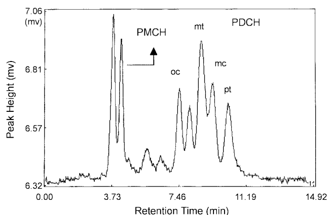
Figure 6. A typical chromatogram of PFCs collected in ambient air.
