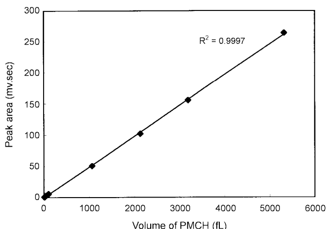
Figure 5. Calibration curve of PMCH standard gas.
