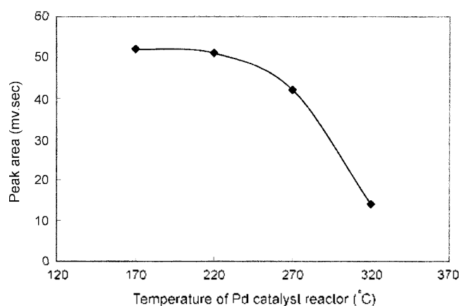
Figure 3. Variation of PMCH peak areas depending on the temperature of Pd catalytic reactor.
