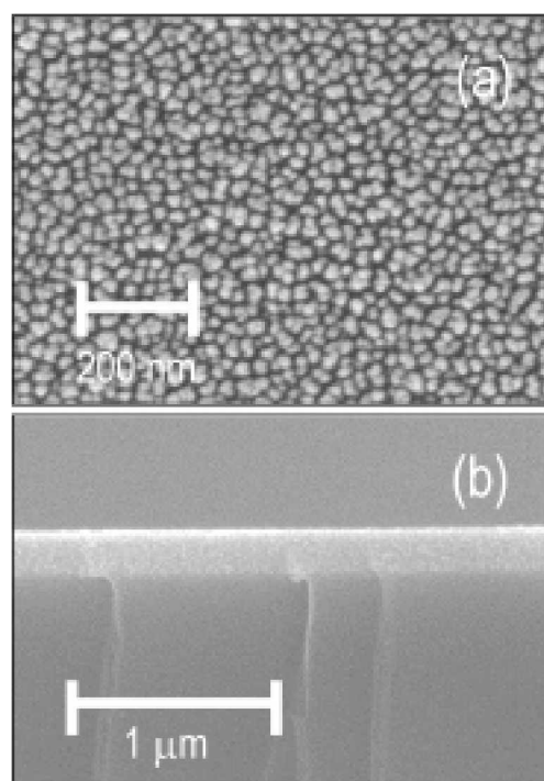
Figure 2. Plan-view (a) and cross-sectional (b) SEM images of the Ga 2 O 3 film of Figure 1.
