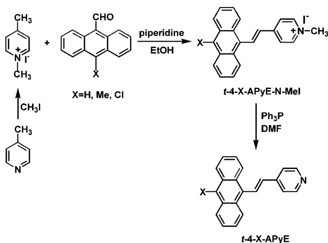
Scheme 2. Synthesis of t -4-X-APyE and t -4-X-APyE-N-MeI.
