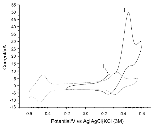
Figure 4. Cyclic voltammetry of the FePc-adsorbed electrode with (solid line) and without (dotted line) \text{SO}_2 in a pH 5 solution. C_{\text{SO}_2} = 2.0 \text{ mM} , scan rate = 0.2 \text{ V}\cdot\text{s}^{-1} . Apparent electrode area = 0.04 \text{ cm}^2 .
