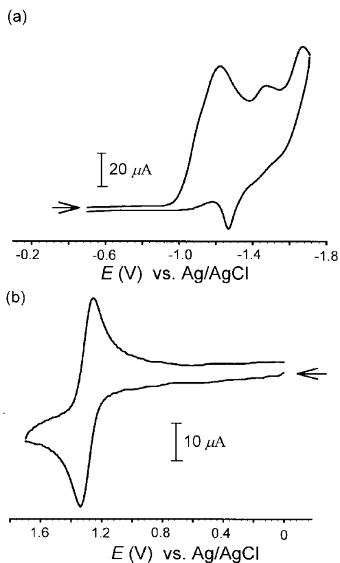
Figure 4. Cyclic voltammogram of (a) a ligand-based and (b) a reversible Fe III/II couple of monomeric [Fe(3-Br-phen) 3 ] 2+ on glassy carbon electrode. Electrolyte solution: 0.1 M TBAH/CH 3 CN. Scan rate; 100 mV · s -1 .
