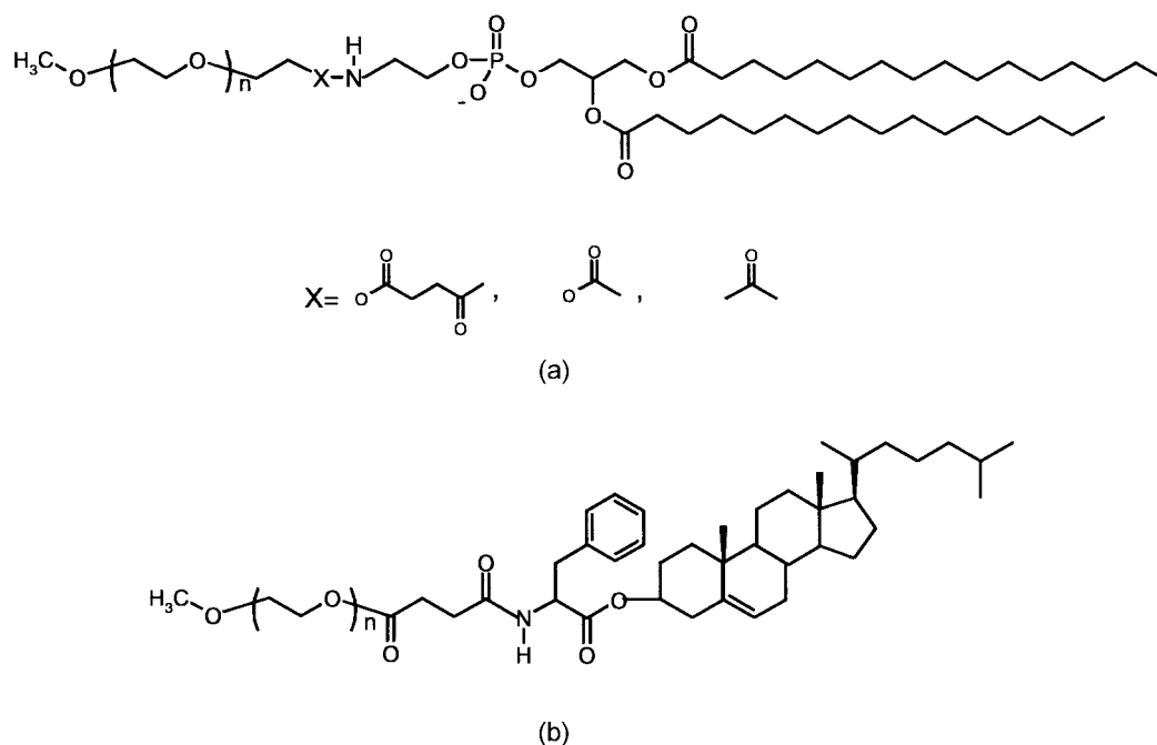
Figure 1. Chemical structures of (a) PEG-DPPE and (b) PEG-Phe-Chol.
