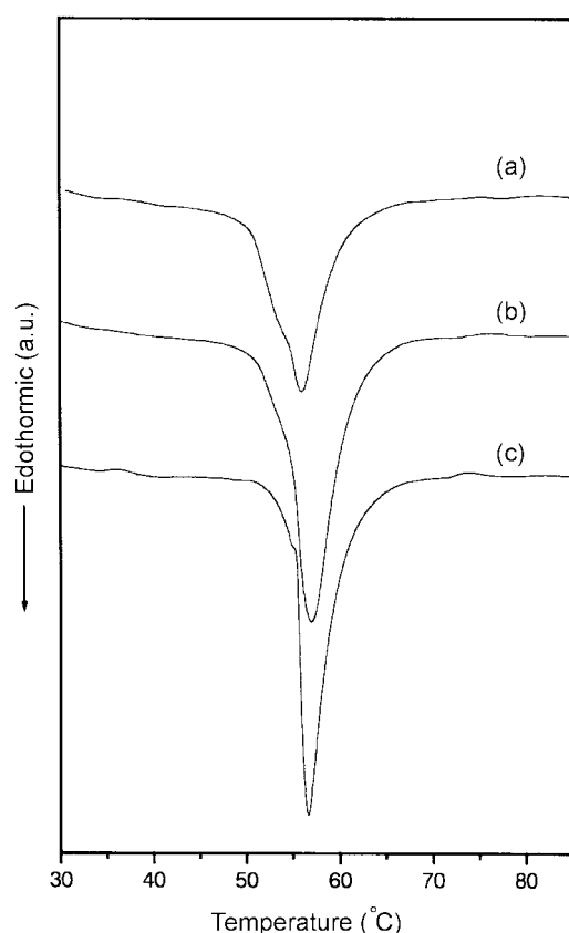
Figure 3. DSC thermograms of hydrated bilayers in PBS (about 50 wt%) of (a) DSPC only, (b) DSPC/PEG-Phe-Chol (95/5), and (c) DSPC/PEG-Phe-Chol (90/10). All of the thermograms were obtained from the second heating scans and the scan rate was 5 °C/min.
