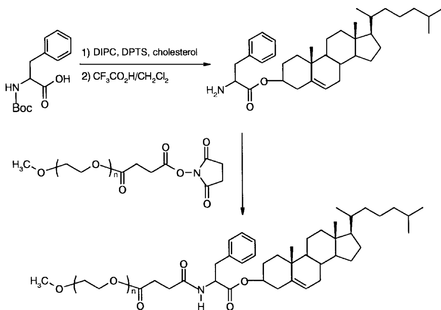
Scheme 1. A chemical synthetic route of PEG-Phe-Chol.
