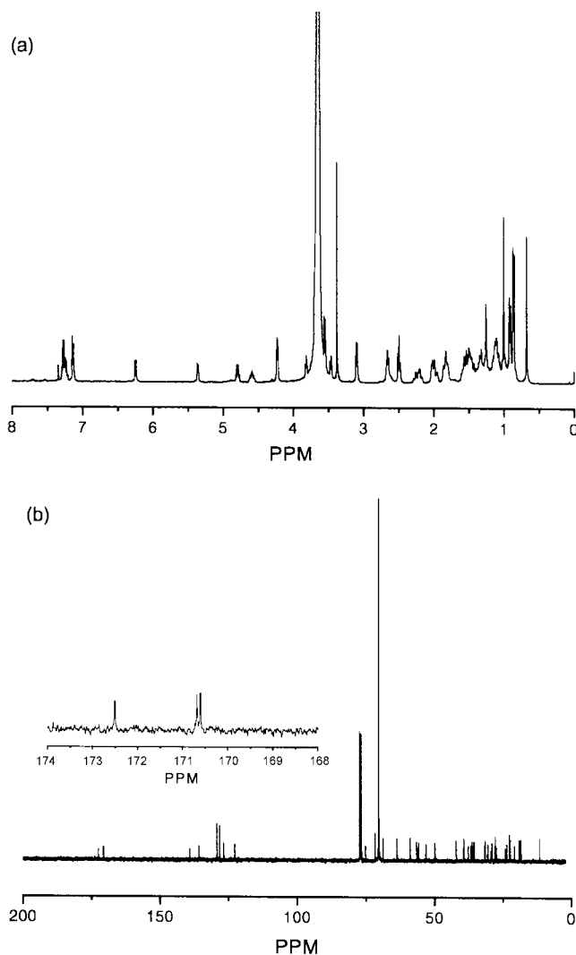
Figure 2. (a) 1 H and (b) 13 C NMR spectra of PEG-Phe-Chol in CDCl 3 (400 MHz).
