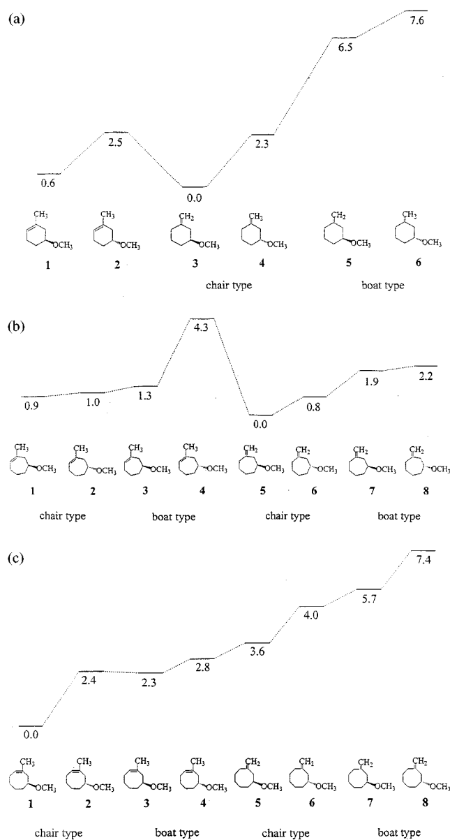
Figure 1. Three schematic potential energy diagrams and optimized structures of the structural isomers of the 6-, 7-, and 8-membered cyclic compounds at the MP2/6-311+G** level. (a): Relative potential energies of the 6-membered cyclic compounds. (b): Relative potential energies of the 7-membered cyclic compounds. (c): Relative potential energies of the 8-membered cyclic compounds. All energies are adiabatic values and are in units of kcal/mol.
