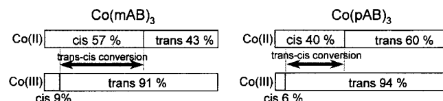
Fig. 3. Trans/cis molar ratio at the photostationary state upon irradiation with monochromatic 366 nm light for the cobalt complexes.
