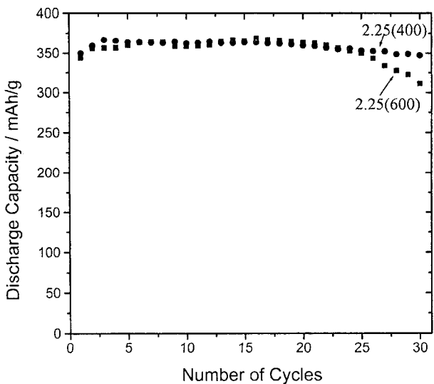
Fig. 6. Cycling performance of 2.25(400) and 2.25(600) electrode (electrolyte : 1 M LiPF 6 /EC:PC:DMC(1:1:3), rate : C/5).
