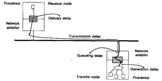
Fig. 1. CAN communication model
