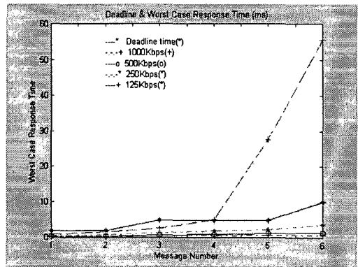
Fig. 3. The performance analysis of the initial CAN-based control system for an AGV with a manipulator arm
