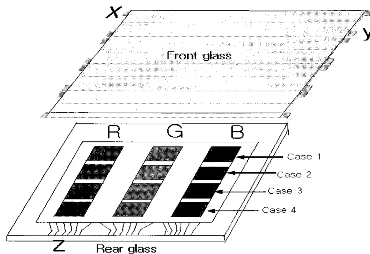
Fig. 1. Schematic diagram of 7-inch AC-PDP test panel with four different phosphor layer patterns.
