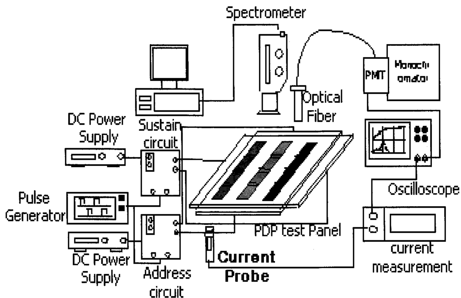
Fig. 2. The schematic diagram of measurement equipment.
