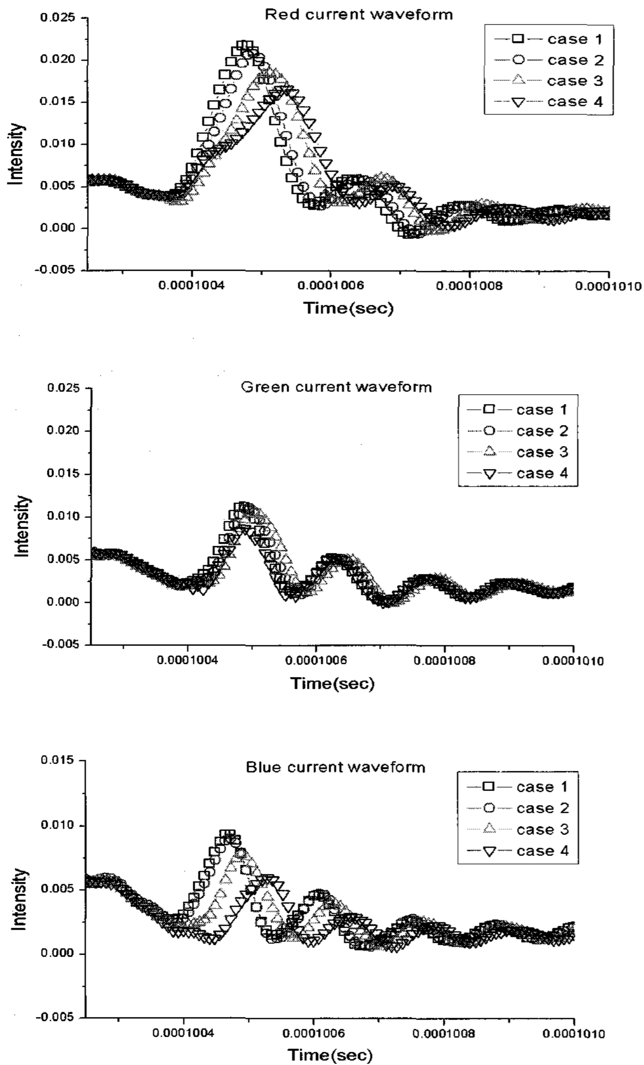
Fig. 7. Changes in discharge current waveforms.
