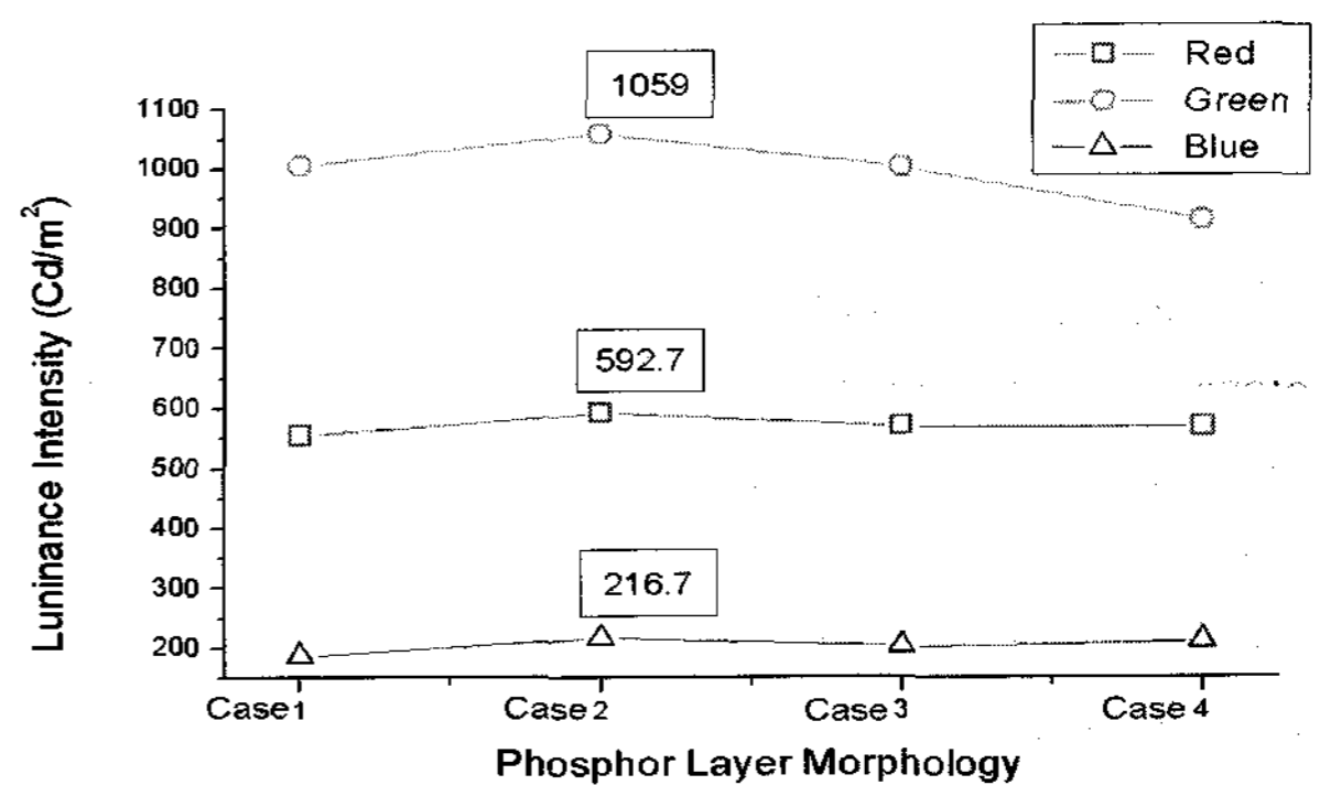
Fig. 8. Changes in luminance of R, G, and B cells.
