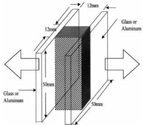
Figure 4. Sample for adhesion force measurement (KS F 4910).
