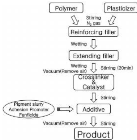
Figure 2. Method of silicone sealant blending.
