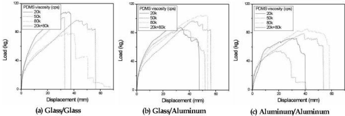
Figure 6. Adhesion force by substrate as a function of PDMS viscosity.
