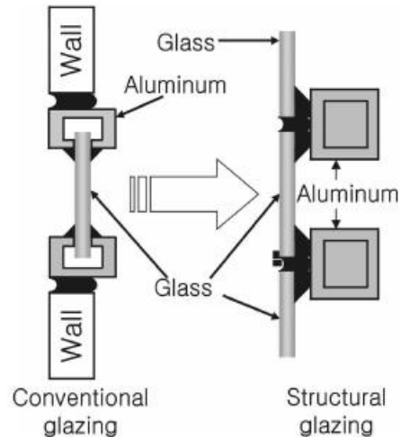
Figure 1. Comparative between conventional glazing and structural glazing.
