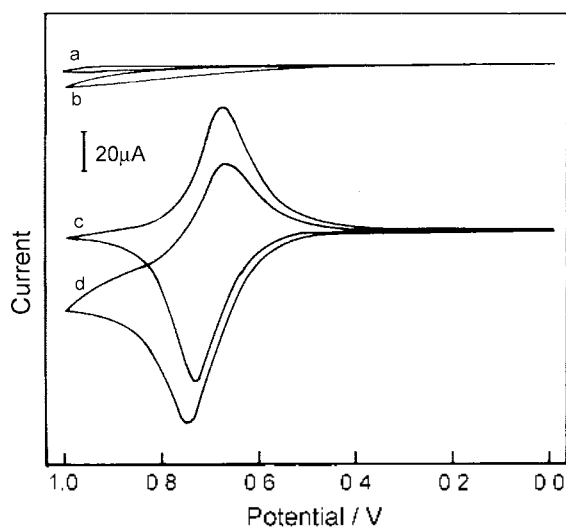
Figure 3. Cyclic voltammograms of (a) bare electrode, (b) 8.1 \times 10^{-4} M GSH at bare electrode, (c) CuHCF modified electrode and (d) 8.1 \times 10^{-4} M GSH at modified electrode; Supporting electrolyte : 0.1 M KNO 3 ; pH 6.5 (0.05 M phosphate buffer); Scan rate: 20 mV/s.
