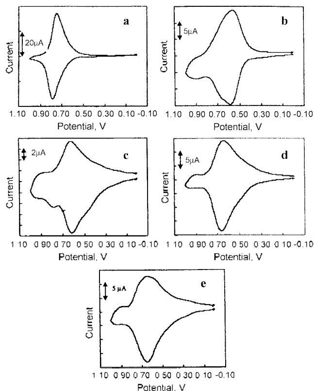
Figure 2. Cyclic voltammograms of CuHCF modified electrode in 0.1 M solution of (a) NH 4 Cl, (b) NaCl, (c) LiCl, (d) BaCl 2 and (e) CaCl 2 ; Scan rate: 10 mV/s.
