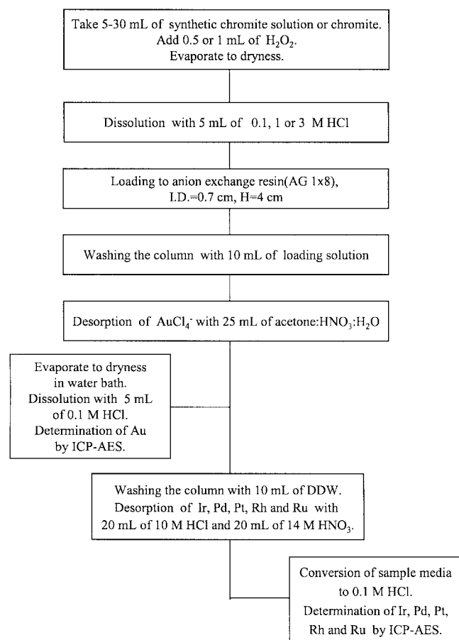
Figure 4. Analytical scheme for Au, Ir, Pd, Pt, Rh and Ru separation.
