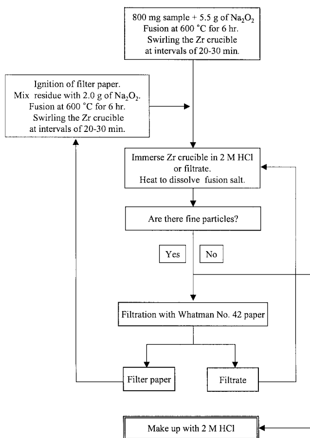
Figure 1. Fusion dissolution procedure for 0.8 g chromite sample.
