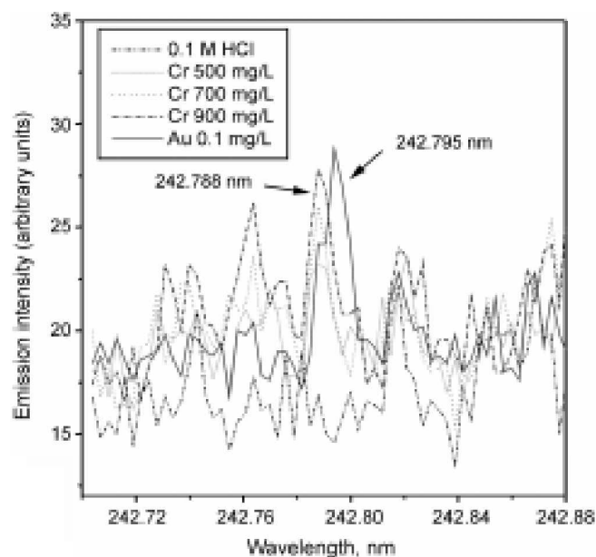
Figure 2. Spectral interference of Cr on Au 242.795 nm.
