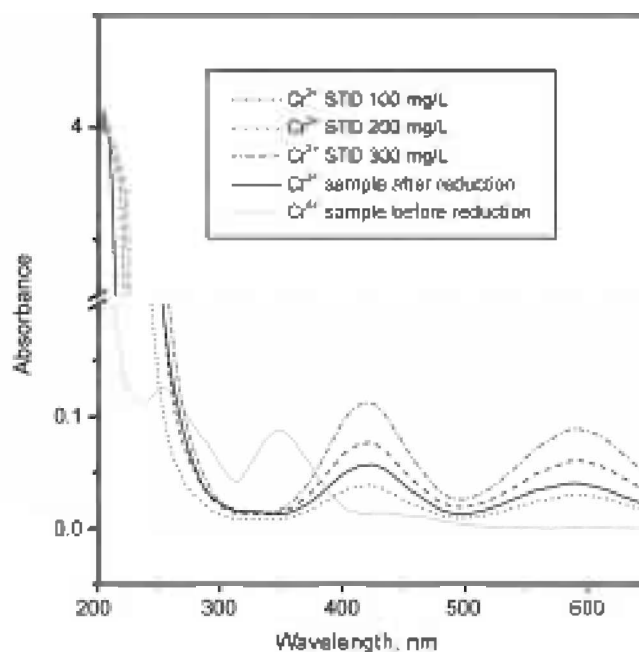
Figure 3. Absorption spectra of Cr 3+ and Cr 6+ solution.
