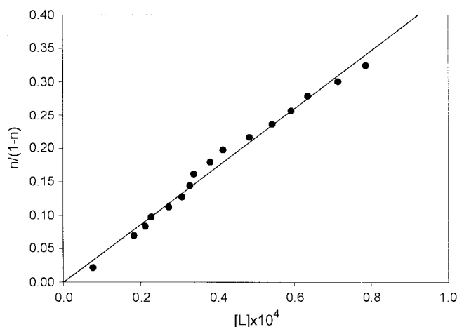
Figure 1. Plot of \bar{n}/(1-\bar{n}) vs [L] for Cu 2+ -L-proline.
