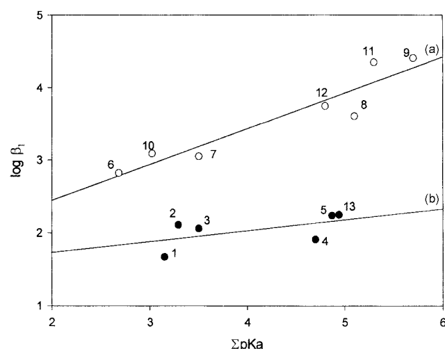
Figure 1. Correlation of \log \beta_1 of the \text{Eu}^{3+} complexes and \Sigma \text{pKa} of the ligand, (a) bidendate (b) monodendate; 1. furoic acid, 2. thioglycolate, 3. methoxyacetate, 4. acetate, 5. propionate, 6. pyrazine carboxylate, 7. \alpha -picolinated N-oxide, 8. \alpha -picolinate, 9. 1,4-cyclohexanedicarboxylate, 10. croconate, 11. malonate, 12. glutarate, 13. cyclopentanecarboxylate
