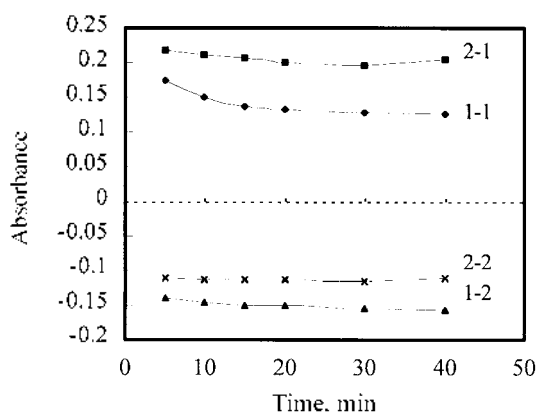
Figure 6. Effect of the reaction time: 1-1 \Delta A of Fe(20 \mu\text{g} )-BBTAN solution at 540 nm and 2-1 \Delta A of Zn(10 \mu\text{g} )-BBTAN solution at 580 nm, 1-2 \Delta A of Fe(20 \mu\text{g} )-BBTAN solution at 460 nm and 2-2 \Delta A of Zn(10 \mu\text{g} )-BBTAN solution at 460 nm, all against reagent blank.
