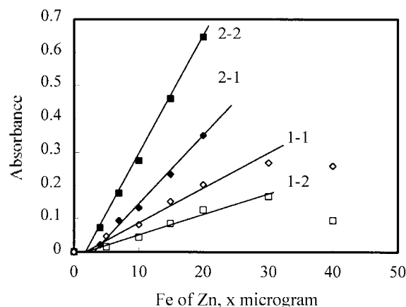
Figure 7. Standard curves for the determination of Fe(II) and Zn(II) at pH 8.5 and in the presence of triton X-100: 1-1- A_\beta of Fe-BBTAN at 540 nm, 1-2- A_\beta of Fe-BBTAN at 580 nm, 2-1- A_\beta of Zn-BBTAN at 540 nm, 2-2- A_\beta of Zn-BBTAN at 580 nm.
