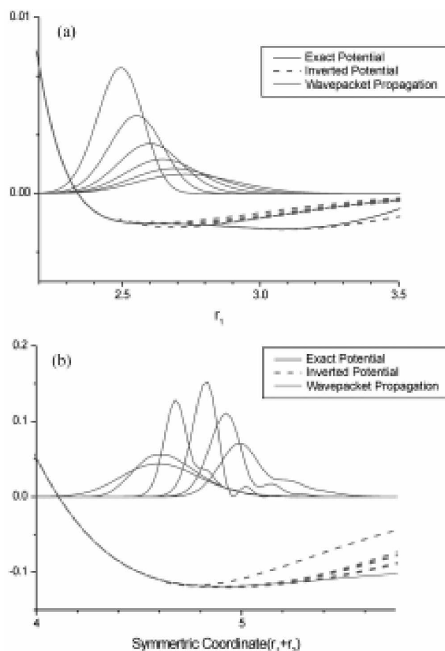
Figure 5. The comparison of the inverted potentials at a certain evolution time (0, 10, 20, 30, 40, 50 fs) with the exact one according to the wave packet propagation. (a) for a fixed value r_2 = 2.4125 a.u. at the equilibrium position of S_1 surface ( \theta = 133.89^\circ ). (b) for a fixed value symmetric coordinate r_1 - r_2 = 0 .
