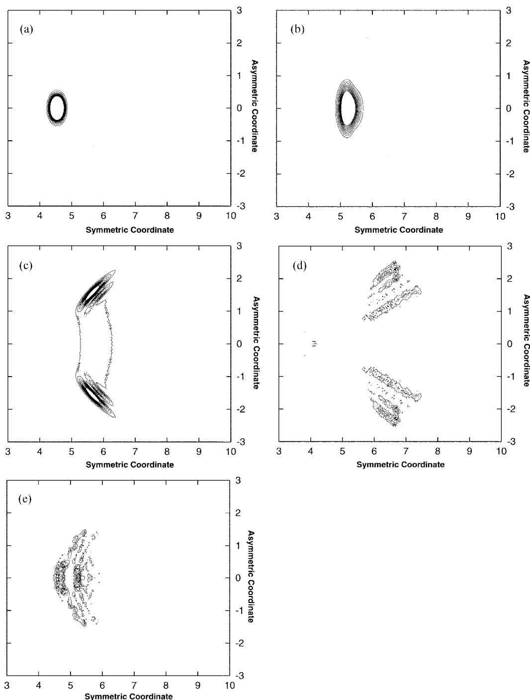
Figure 2. the wave packet \psi(t) as a function of the symmetric stretch coordinate r_1 + r_2 and asymmetric stretch coordinate r_1 - r_2 at (a) 0, (b) 12, (c) 24, (d) 48 and (e) 120 fs ( \theta = 133.89^\circ ).
