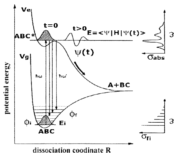
Figure 1. The UV photodissociation of triatomic molecule ABC into products A+BC . The electronic excitation occurs from the molecule in a particular initial state |\phi_i\rangle in the ground electronic state ( S_0 ) to the excited singlet electronic state ( S_1 ). The corresponding PES are V_g and V_e , respectively. \sigma_{abs}(\omega) and \sigma_{fi}(\omega) denote the absorption cross section and the Raman scattering cross section, respectively. 31
