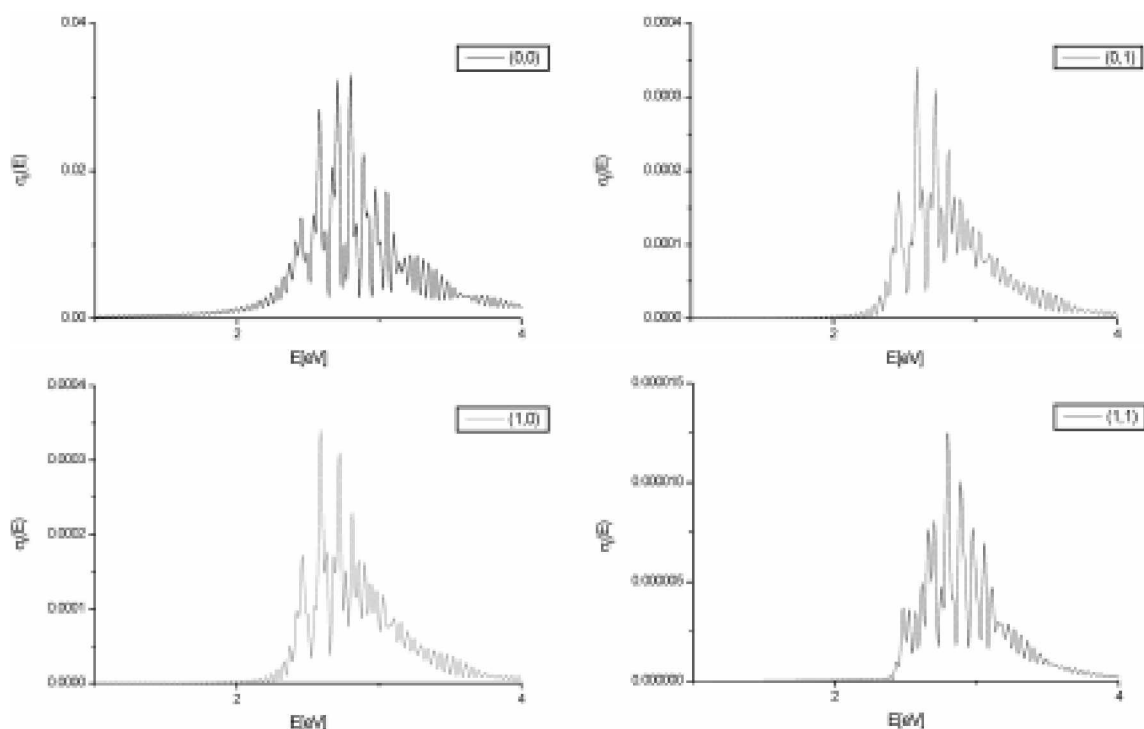
Figure 4. Raman Excitation Profile. \sigma_f(E) , f = (0,0), (0,1), (1,0), (1,1) ( \theta = 133.89^\circ ).
