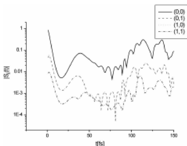
Figure 3. The amplitude of the correlation function ( \theta = 133.89^\circ ).
