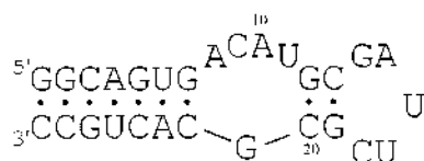
Scheme 1. Secondary structure and numbering of the RNA.
