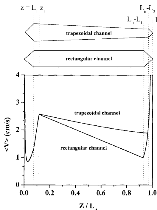
Figure 5. Comparison of linear flow velocities in trapezoidal and rectangular channels. Flow rate conditions are \dot{V}_s = 0.15 , \dot{V}_f = 2.4 , \dot{V}_c = 1.69 , and \dot{V}_{out} = 0.86\text{ mL/min} . The channel dimensions used for calculation: Trapezoidal L_1 = 2.0 , L_2 = 1.0 , b_1 = 2.0 , b_2 = 1.0 , z_1 = 3.1 , L_n = 27.2\text{ cm} , and w = 78.3\text{ }\mu\text{m} ; Rectangular L_1 = L_2 = 2.0\text{ cm} and b_1 = b_2 = 2.0\text{ cm} with all other dimensions as for trapezoidal channel. [Reprinted with permission from Anal. Chem. 1997 , 69(7) 1438. Copyright 1997 American Chemical Society]
