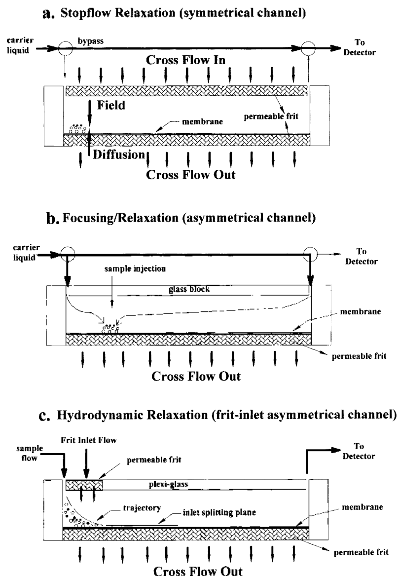
Figure 2. Side views of three different flow FFF channels (a. symmetrical, b. asymmetrical, c. frit-inlet asymmetrical channel) showing the flow direction during sample relaxation (bold lines) and during separation (solid lines).
