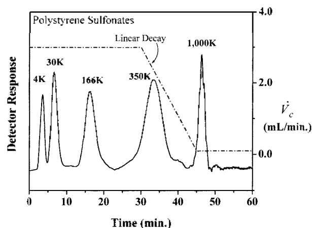
Figure 11. Separation of PSS standards with field programming ( t_1 = 30 min, t_p = 15 min, \dot{V}_{c0} = 3.0 mL/min, \Delta \dot{V}_c = 2.9 mL/min) obtained at \dot{V}_s = \dot{V}_{out} = 0.10 mL/min. The run is made at \dot{V}_f = \dot{V}_c during programming. System II with YM-10 membrane is used.
