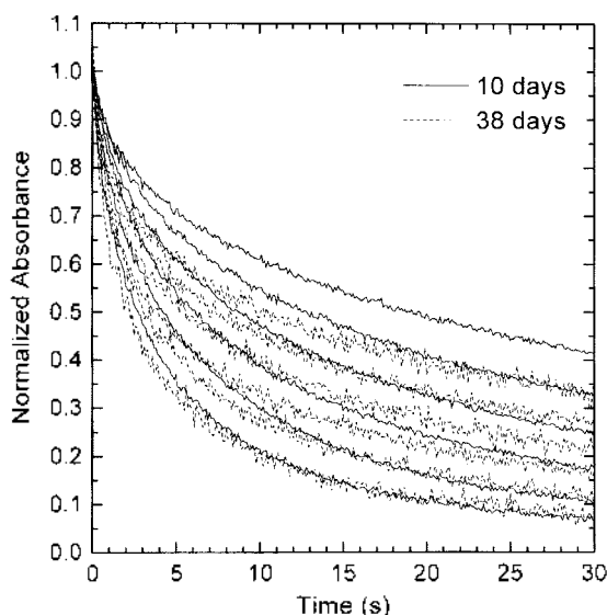
Figure 2. Aging effects on the thermal bleaching reaction of PMC in PS at various temperatures. Probe wavelength was 594 nm. Temperatures of the sample are 298 K, 293 K, 288 K, 283 K, 278 K, and 273 K from the bottom for each set of data.
