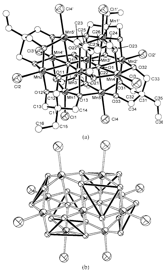
Figure 1. (a) ORTEP diagram of [Mn 10 O 2 Cl 8 {(OCH 2 ) 3 CCH 2 -CH 3 } 6 ] 2- ( 1 ) showing the 50% probability thermal ellipsoids. Hydrogen atoms and counter ions are omitted for clarity. (b) Schematic representation of the [Mn 10 L 28 ] core, highlighting the triangular cavities available for occupancy by the oxygen donors of trisalkoxy ligands.
