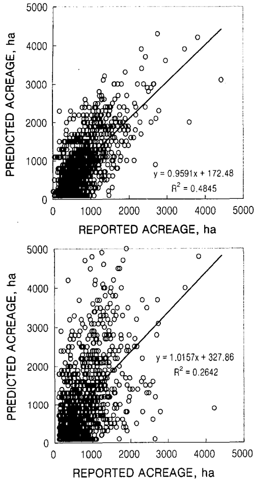
Fig. 2. Rice acreage of each Myeon, which is estimated by counting the pixels classified as rice paddies by our method (upper) and by the USGS method (lower), is plotted against the reported acreage.
