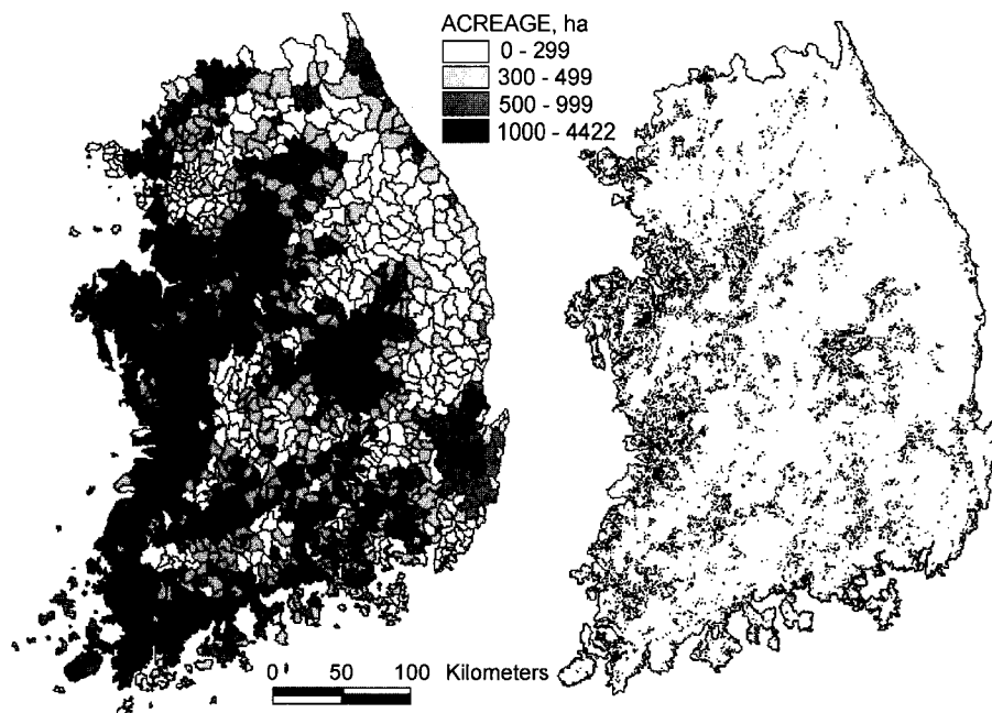
Fig. 1. Distribution pattern of rice paddies across South Korea predicted by NOAA-AVHRR data analysis (right). Reported acreage of each Myeon is also shown for comparison (left).
