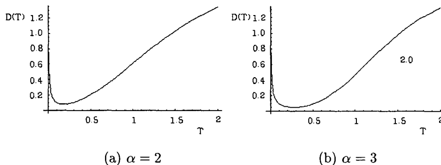
Figure 3. Optimal inspection period based on minimum D(T)
