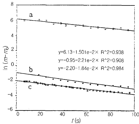
Figure 4. Plots for first order reactions time dependence of frequency changes of a quartz crystal resonator for the polymerization reaction kinetics of [Ru(v-bpy) 3 ] 2+ (A), vba(B), and 1:1 mol ratio of two compounds (C).
