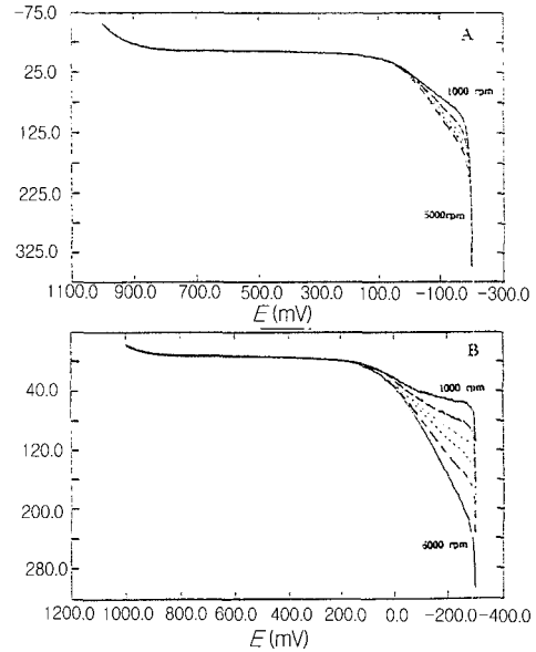
Figure 5. Rotating disk voltammograms of Pt/p-[Ru(v-bpy) 3 ] 2+ /vba(A) and Pt/p-[Ru(v-bpy) 3 ] 2+ /vba-dopamine(B) electrode in phosphate buffer (pH= 7.10).
