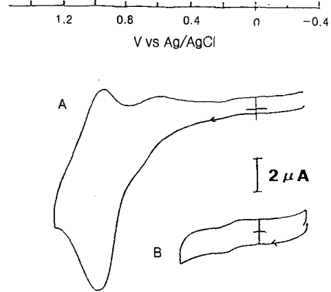
Figure 2. Cyclic voltammograms of GC/p- [Ru(v-bpy)_3]^{2+}/vba(5:2) modified with dopamine at scan range of -0.30 to 1.30 V(A), and -0.3 to 0.60 V(B) in phosphate buffer (pH=7.10).
