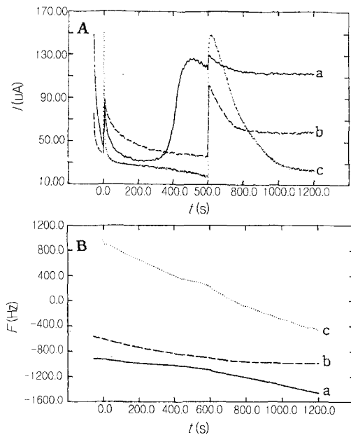
Figure 3. (A) is Chronoamperograms of electropolymerization for (a) [Ru(v-bpy)_3]^{2+} , (b) vba, and (c) 5:2 mol ratio of two compounds, (B) is time dependence of frequency changes of a quartz crystal resonator for Figure 3(A) respectively.
