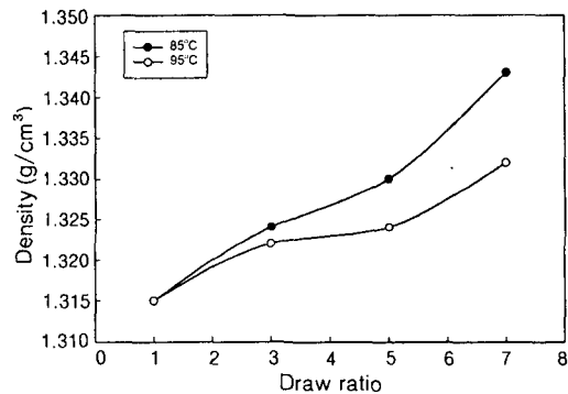
Figure 4. Plots of density vs. draw ratio for PET/BPA copolymer films drawn at draw rate 0.1 cm/min and draw temperatures as indicated.
