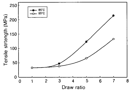
Figure 11. Plots of tensile strength vs. draw ratio for PET/BPA copolymer films drawn at draw rate 0.1 cm/min and draw temperatures as indicated.
