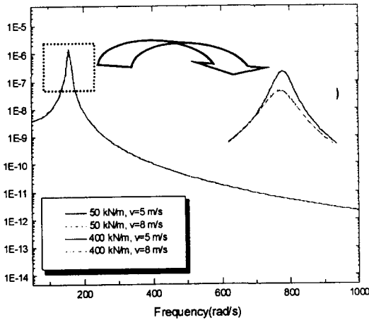
Fig. 5. Frequency Response Function for Spring Support
