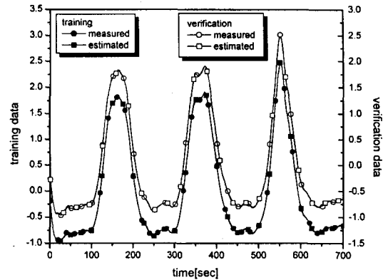
Fig. 6. Estimation of a (standardized) Pressurizer Pressure Signal Using the PGP Method
