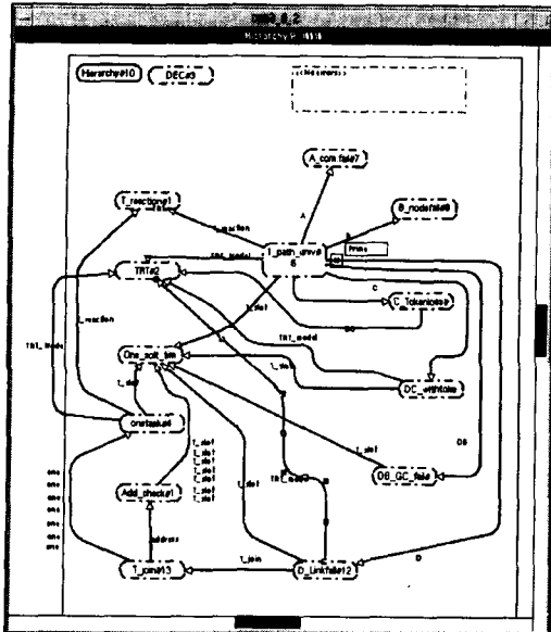
Fig. 5. CPN Hierarchy Page for 1_path TCD
