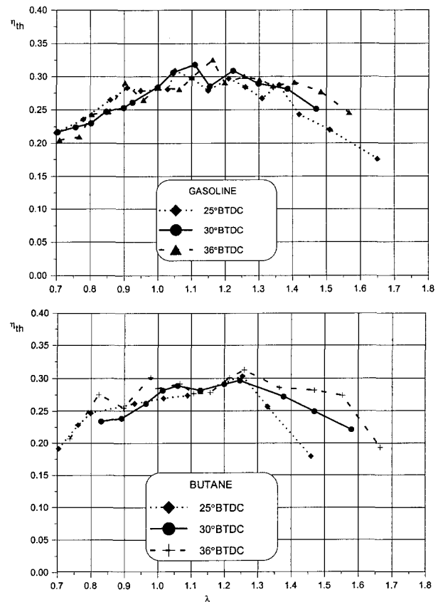
Figure 10. Engine thermal efficiency as a function of air excess coefficient \lambda for three ignition timings and for fuelling with gasoline and gaseous butane. Conditions as in Fig. 9.
