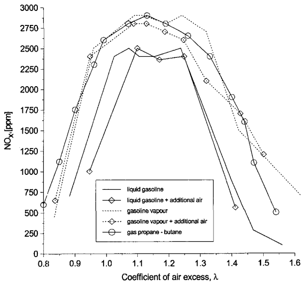
Figure 5. NO x emission as a function of air excess coefficient \lambda for conditions as in Fig. 3.
