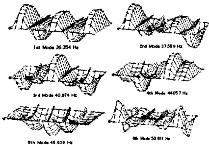
Fig. 3: The natural mode of NR45 model (1st-6th)
