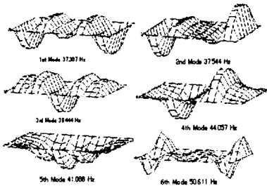
Fig. 8 : The natural mode of NR5B model (6 at=60)
