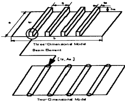
Fig. 7 : Two-Dimensional model for analysis
