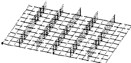
Fig. 2(b): Stiffened plate NR510 model for FEM analysis
