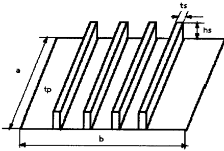
Fig. 1: Stiffened plate model for analysis
