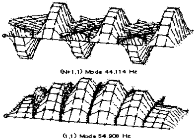
Fig. 6 : The main mode of NR510 model
