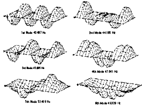
Fig. 9 : The natural mode of NR510B model (1st=90)
