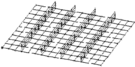
Fig. 2(a): Stiffened plate NR45 model for FEM analysis
