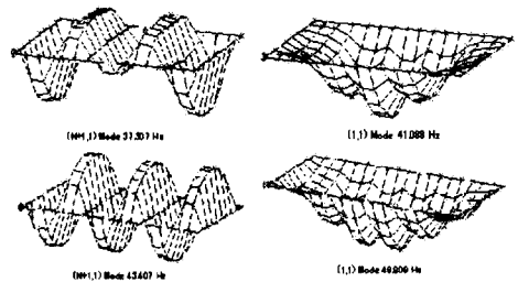
Fig. 10 : The main mode of NR45B & NR510B model
