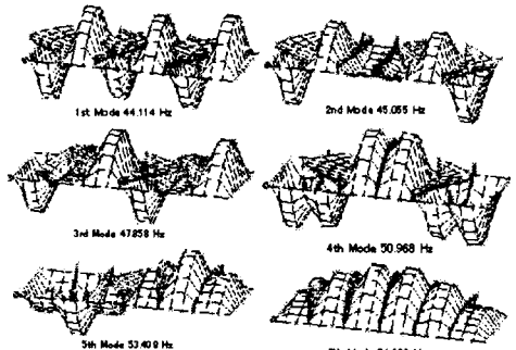
Fig. 5: The natural mode of NR510 model (1st-8th)
