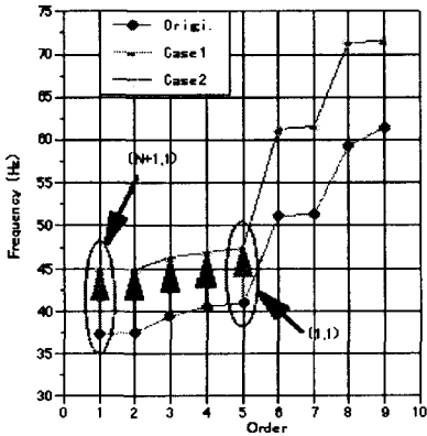
Fig. 11 : Comparison of natural frequency Case1 & Case2
