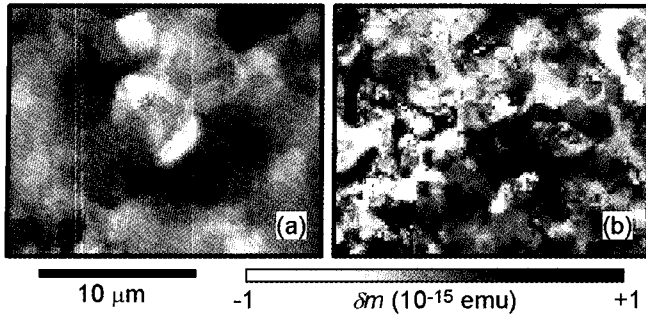
Fig. 3. Spatial distribution of the activation magnetic moment of (2.5\text{-}\text{Å}\text{ Co}/11\text{-}\text{Å}\text{ Pd})_n multilayer samples with different number of repeats n = (a) 5 and (b) 15, respectively. The deviation \delta m of the activation magnetic moment from the mean value was mapped onto the corresponding pixel having unit size of 0.4 \times 0.4 \mu\text{m}^2 as a gray level given by the pallet bar at the bottom of the figure. Each map corresponds to a sample surface area of 20 \times 16 \mu\text{m}^2 .
