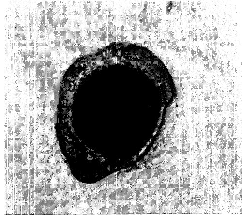
Fig. 1. A hole drilled by 1064 nm pulsed Nd:YAG laser.
