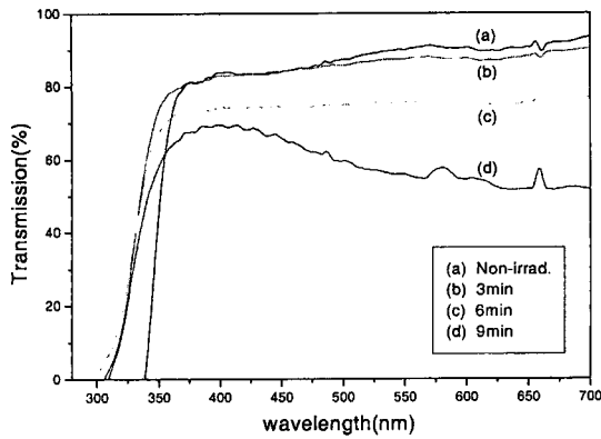
Fig. 3. Glass transmission spectra after laser irradiation with 355 nm wavelength for various time.
