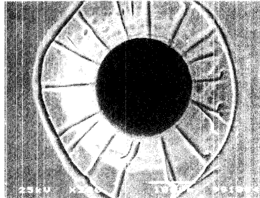
Fig. 2. SEM photograph of laser drilled hole after polishing of surface covered with slag.
