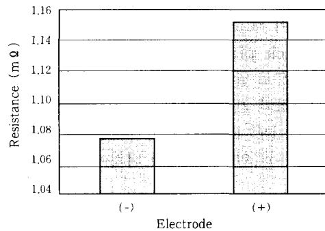
Fig. 12 Comparison of resistance for two welding point (L/R)(Up slope 2ms, Main heat 4ms)
