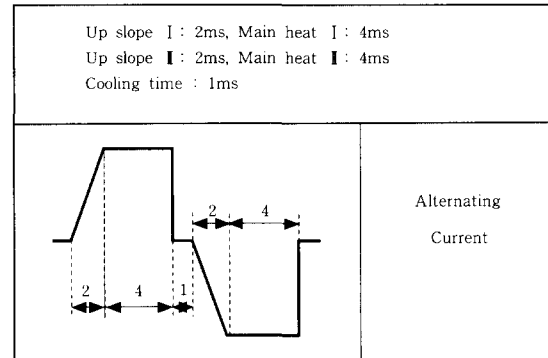
Fig. 5 Schematic diagram for alternating current
