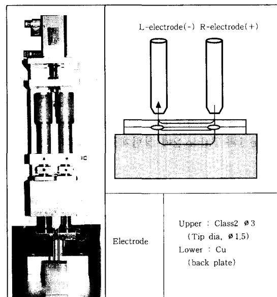
Fig. 6 Appearance of twin head and schematic diagram of electrode for series welding
