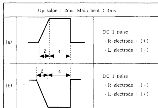
Fig. 3 Schematic diagram of DC 1-pulse for series welding
