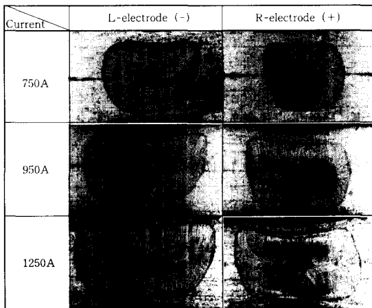
Fig. 10 Growth of nugget by increasing current (34.3N)
