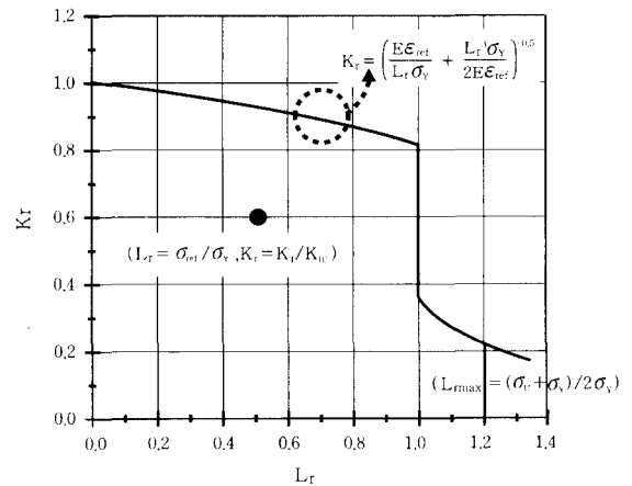
Fig. 4 Level 3 FAD (in this paper)
