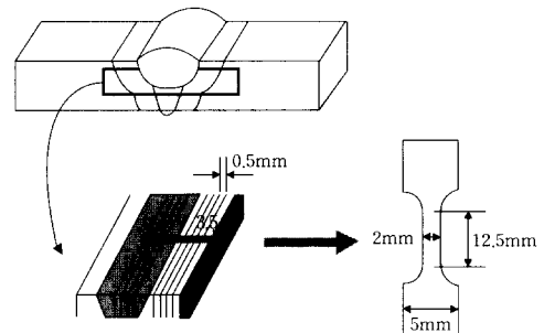
Fig. 9 Micro-tensile specimens used for evaluating tensile properties of HAZ
