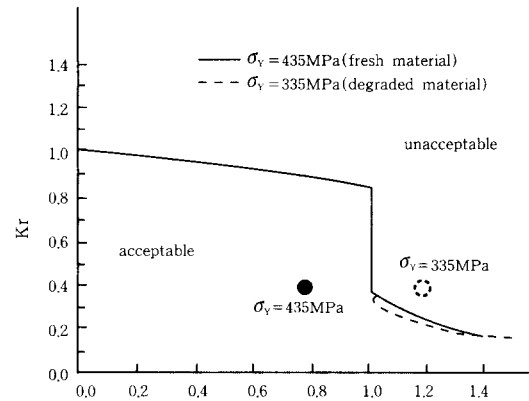
Fig. 8 Difference in assessment result between fresh-material-based FAD and degraded-material-based FAD
