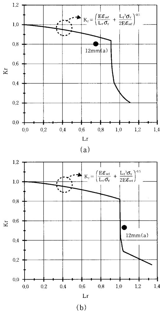
Fig. 7 Difference in FFS assessment result between (a) weld-metal-based FAD and (b) HAZ-based FAD (a: flaw depth)
