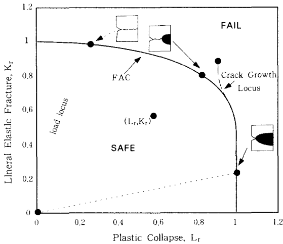
Fig. 1 Typical failure assessment diagram (FAD) 12)
