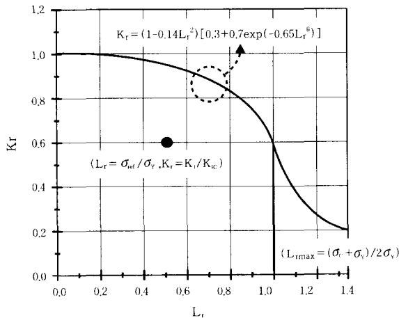
Fig. 3 Level 2 FAD (in this paper)
