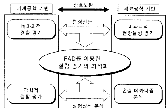
Fig. 11 Various factors for the enhanced fitness-for-service assessment using FAD
