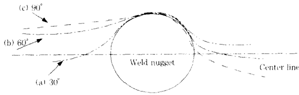
Fig. 8 Crack propagation direction on each IB specimens
