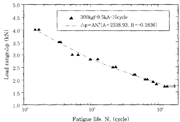
Fig. 3 Fatigue failure life on SPRC35
