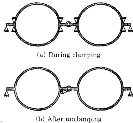
Fig. 10 Boundary conditions for deformation analysis
