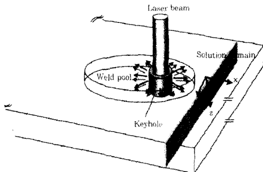
2 Heat flow in the vicinity of keyhole
