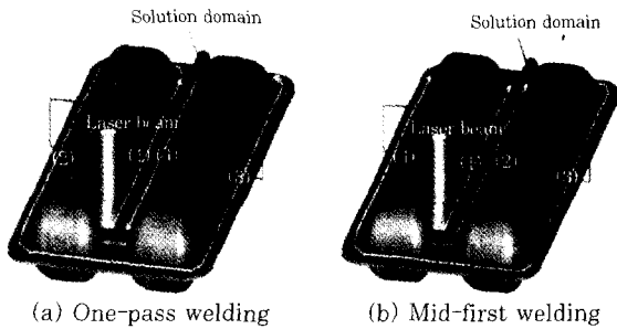
Fig. 8 Welding sequences for the gas vessel
