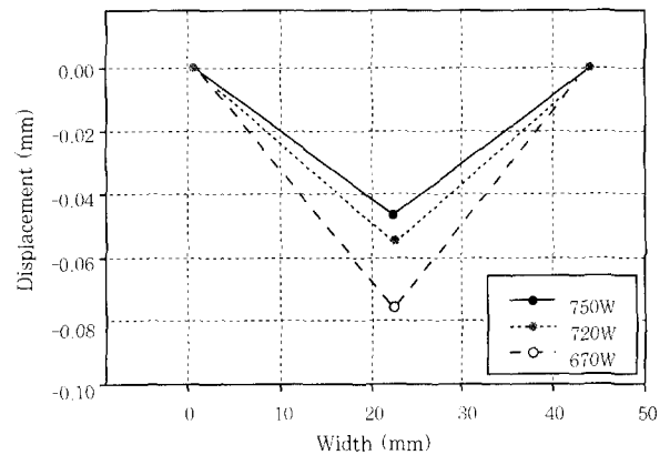
Fig. 15 Calculated displacement of welded vessel in mid-first welding
