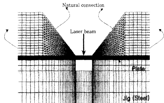
Fig. 5 2-D finite element model of plate welding
